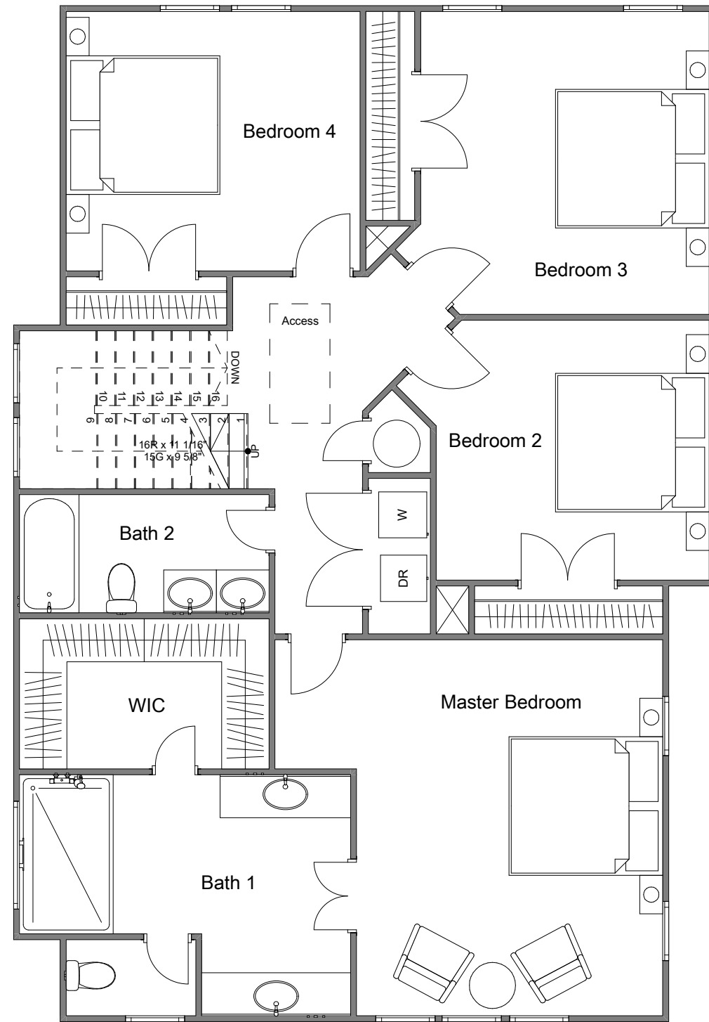
Second Floor
